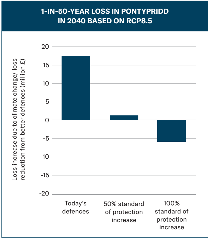
Figure 1: Interplay between increase in loss due to climate change and reduction in loss due to better flood defences.
